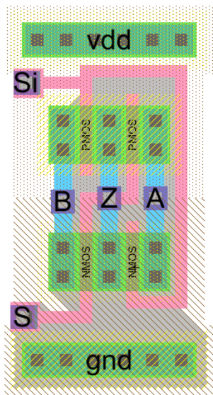
Fig.23. Layout design for2x1 Multiplexer
