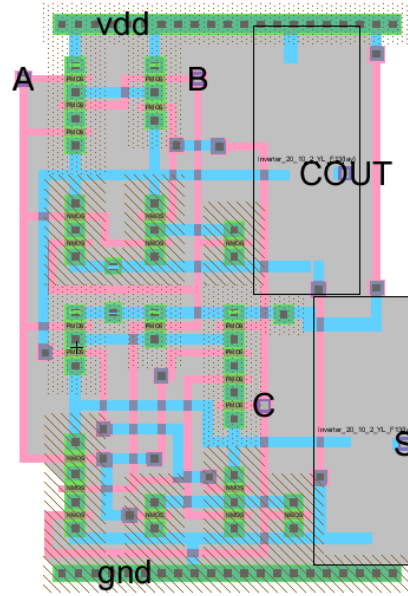
Fig.26. Layout design for Full Adder
