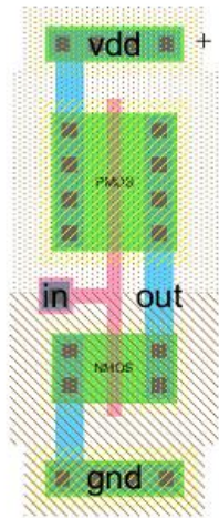
Fig.8. Layout design for inverter (NOT gate)
