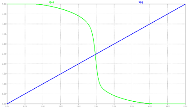
Fig.11. DC Analysis of CMOS Inverter
