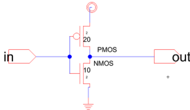
Fig.6. Schematic design for inverter (NOT gate)
