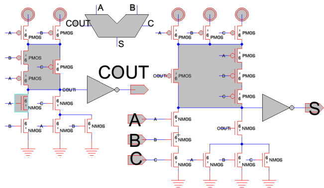
Fig.24. Schematic Design for Full Adder
