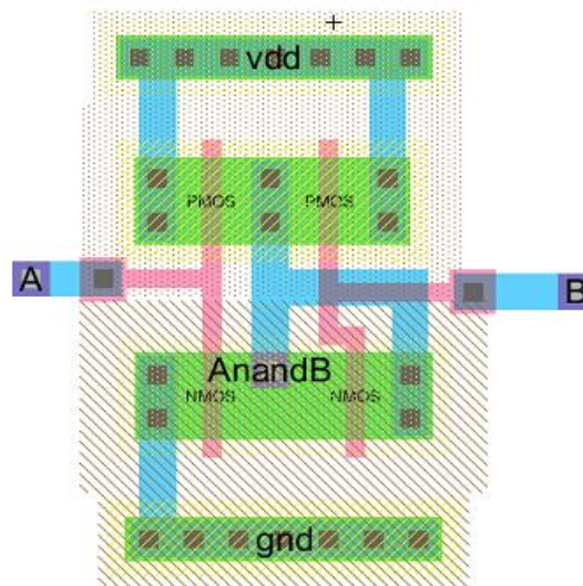
Fig.14. Layout design for NAND gate
