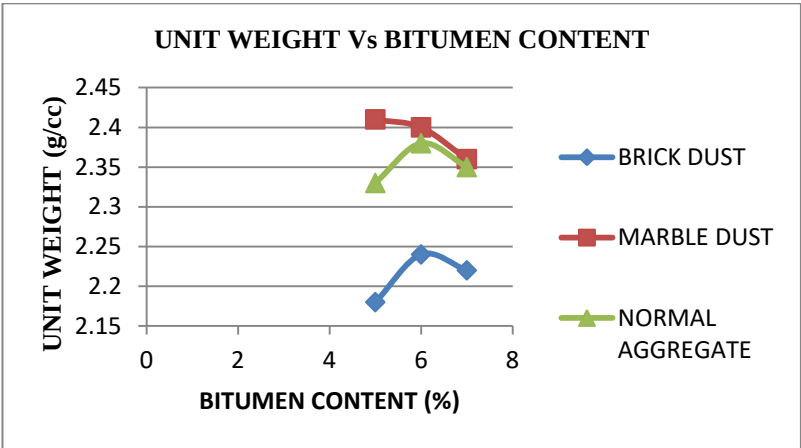
Figure 3: Graph between Bitumen content and Unit Weight
